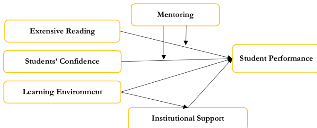
Figure 1: Research Model
